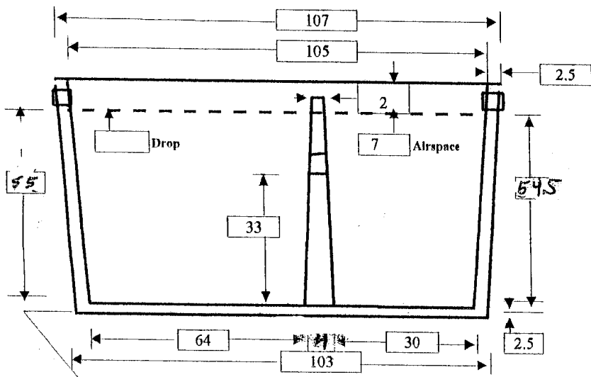
ELEVATION VIEW Show sidewall steel (if any) on this view
