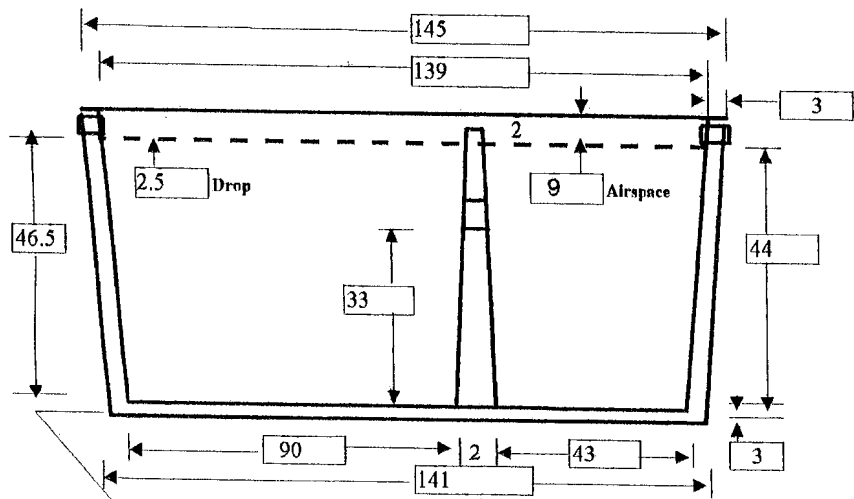
ELEVATION VIEW Show sidewall steel (if any) on this view
