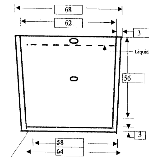
TYPE a END VIEW Show endwall steel (if any) on this view
