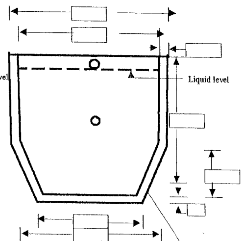
TYPE b END VIEW Show endwall steel (if any) on this view
